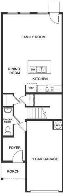
1ST FLOOR PLAN
